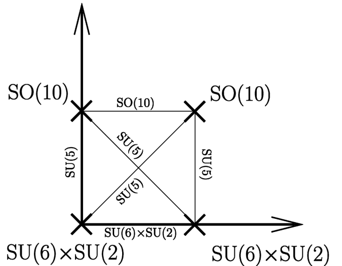
FIG. 10. 6D field theory orbifold picture of gauge symmetry breaking pattern in the SU(5) model. In the bulk there is an \text{SO}(12) \times \text{SU}(2) \times \text{SU}(2) gauge group. Gauge groups written at lines connecting two fixed points are the ones surviving both of the corresponding projection conditions.
